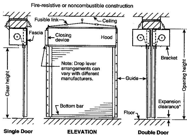
FIGURE A.4.7.5(k) Rolling Steel Doors — Surface Mounted.
