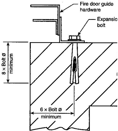
FIGURE A.4.8.6(a) Corner Walls.
